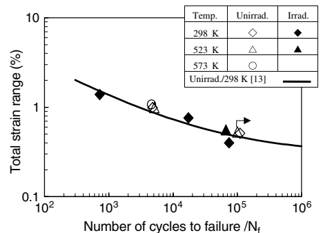
Fig. 3. Total strain range ( \Delta\epsilon_t ) as a function of number of cycles to failure ( N_f ) for unirradiated and irradiated F82H specimens.
